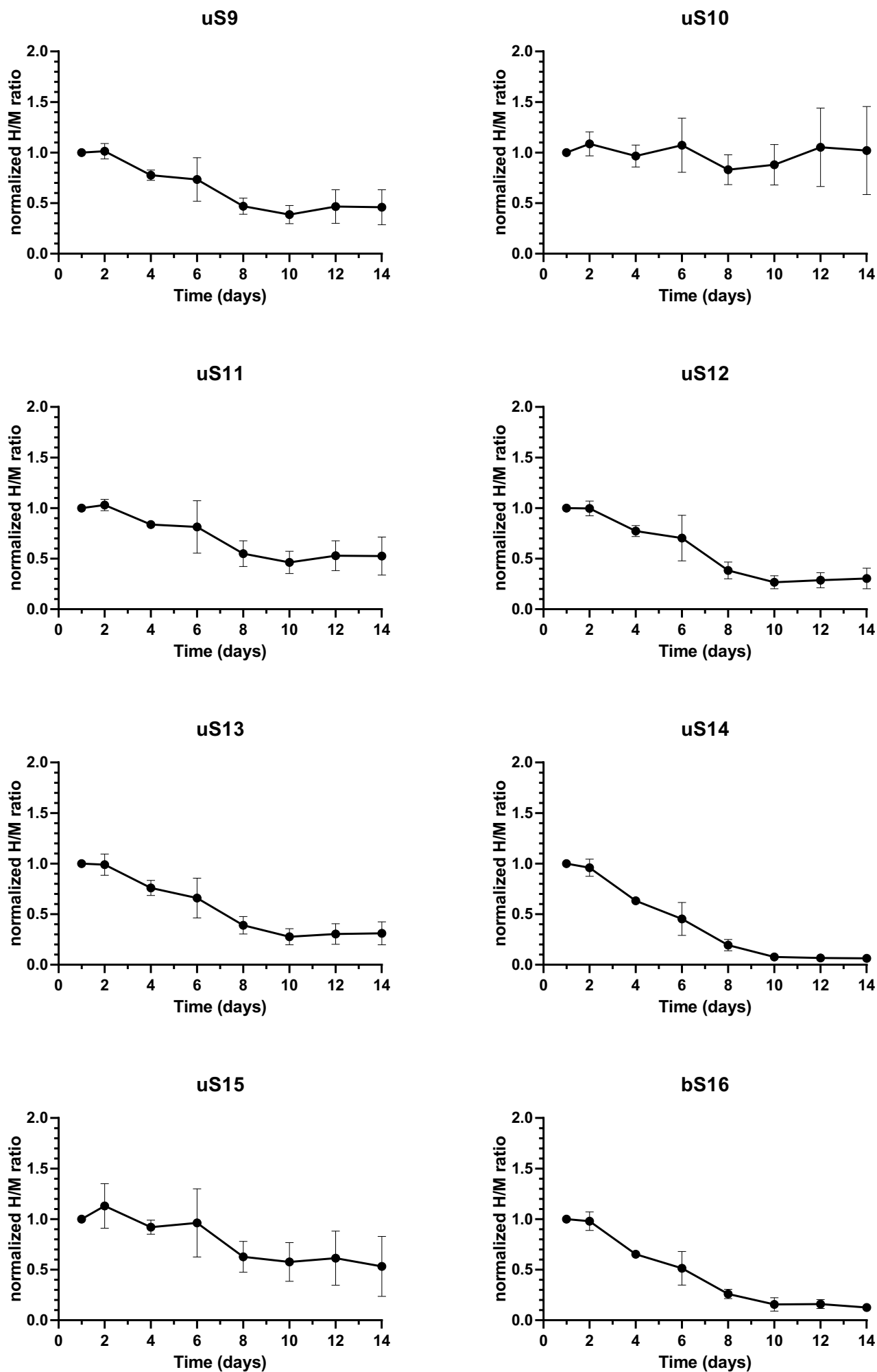
Figure S9 – Individual 30S r-proteins H/M ratio changes in proteome during stationary phase (2/3)
