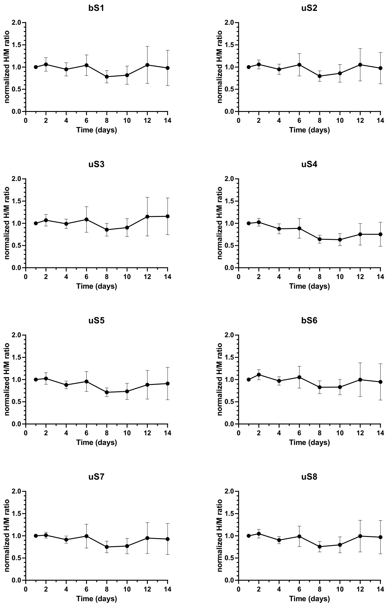
Figure S9 – Individual 30S r-proteins H/M ratio changes in proteome during stationary phase (1/3)
